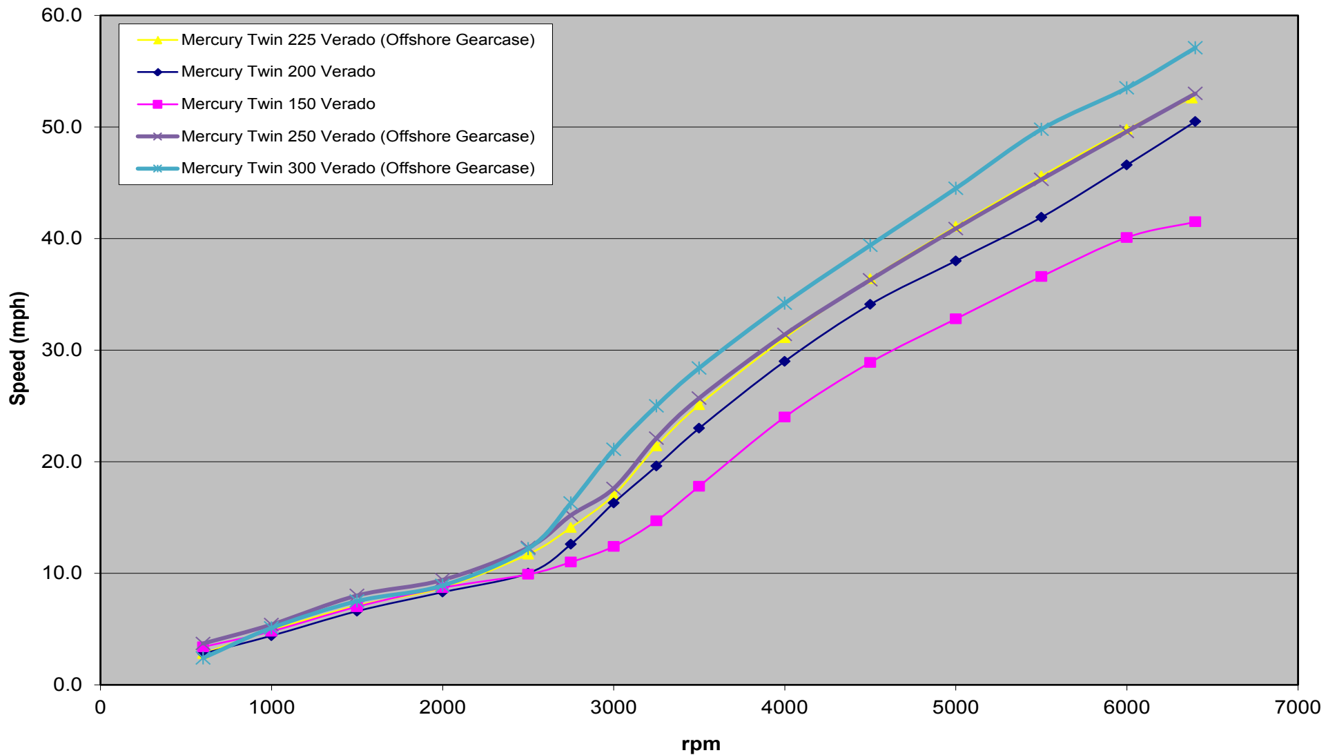
270 Vantage Engine Comparison Graph
