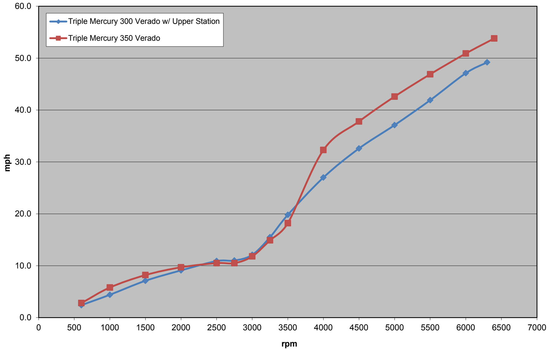
345 Conquest Engine Comparison Graph
