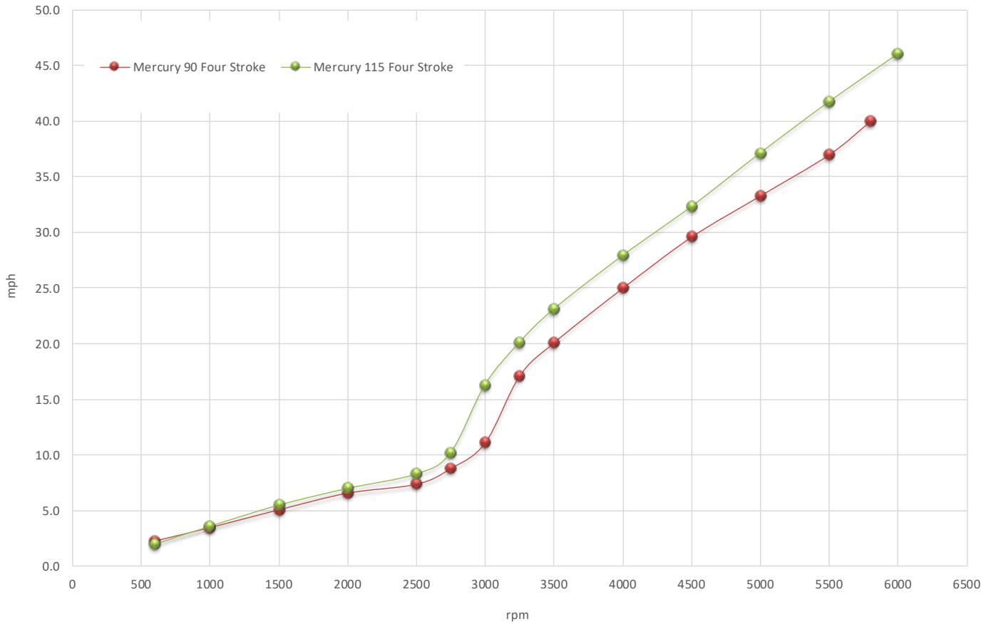
170 Montauk Engine Comparison Graph
