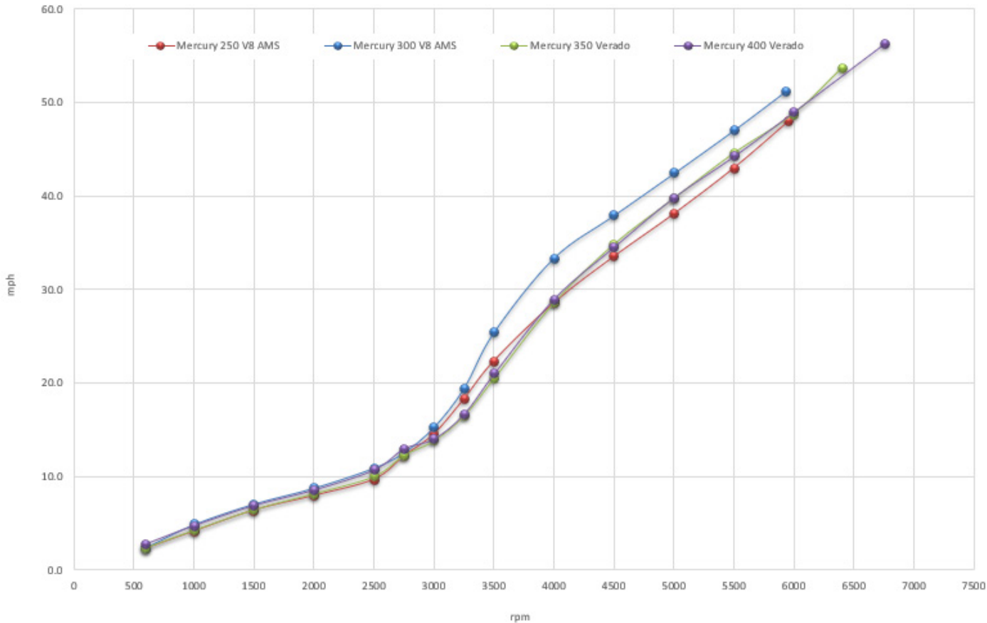
250 Dauntless Engine Comparison Graph
